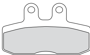
FDB2060 78.7x47x7.4mm
