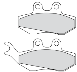
FDB2106 94.6x42x7.6mm
