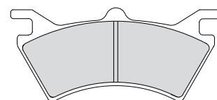
FDB2177 124.4x55.5x10mm
