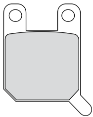
FDB2107 41.3x51.5x6mm
