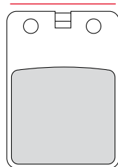
FDB696 43.6x64.6x7mm
