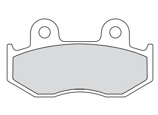
FDB382 81x42x7.5mm
