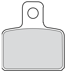
FDB2127 36x39.2x6mm
