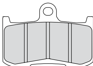
FDB2158 69.8x49.6x7.1mm
