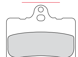
FDB866 56x47x6mm
