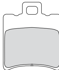
FDB680 39.9x49.6x7mm
