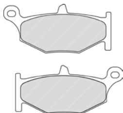
FDB2213 89.4x40.7x9.8mm
