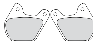
FDB334 71x89x6.5mm
