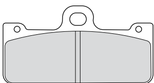
FDB2123 77.8x40.8x10mm
