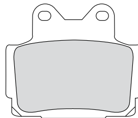
FDB386 66x56x8.8mm
