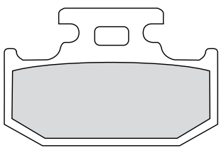
FDB659 62x41x9.4mm
