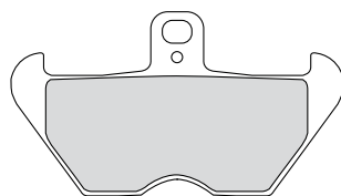
FDB2050 100x55.8x8.4mm
