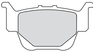
FDB2182 75.4x39.7x9.7mm
