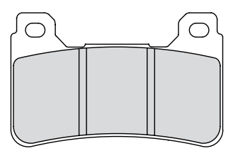
FDB2181 74.6x47.4x8mm
