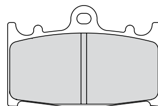
FDB2163 69.9x46.1x13.1mm
