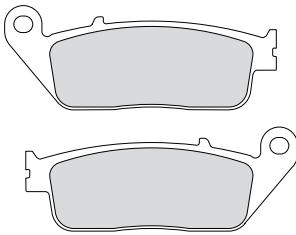
FDB2131 102.3x39.3x9mm
