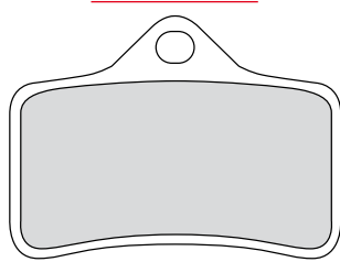
FDB2033 69.6x52.1x8mm
