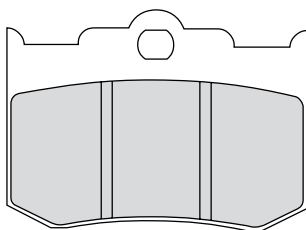
FDB2040 69.4x51.1x7.9mm
