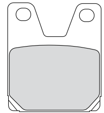
FDB2084 51.9x59.8x8.6mm
