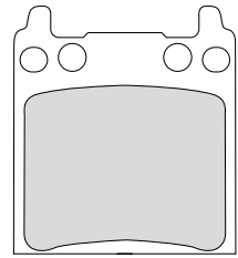
FDB134 58x63x10.4mm
