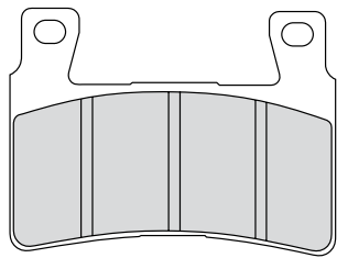
FDB2114 74x55.1x7.1mm
