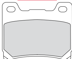
FDB337 63.7x54.5x9.7mm
