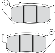
FDB2179 102.1x46.3x8.9mm
