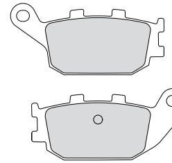
FDB2130 87x40.3x8.9mm
