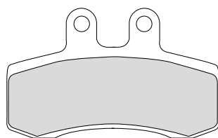
FDB782 87x53x7.5mm
