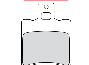
FDB889 39.9x54.1x6.5mm
