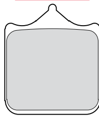
FDB2120 35.2x39.7x7.6mm
