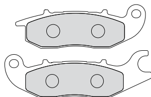
FDB2169 111.4x36.3x7.6mm
