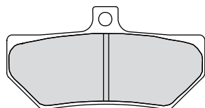
FDB2168 76.6x40.5x8mm
