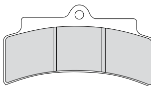
FRP417 102.6x54.5x7mm
