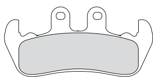
FDB699 100x47x7.5mm
