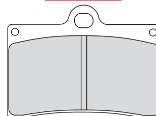
FRP419 69.7x51.4x11mm
