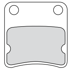
FDB625 41x43x7.7mm
