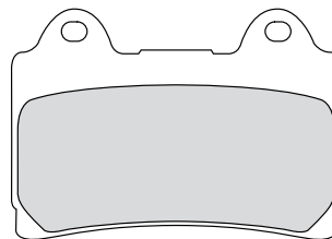
FDB449 75x54x10.7mm
