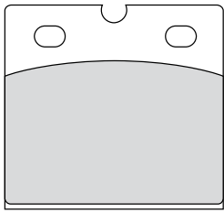
FDB108 56x55x9mm
