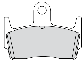
FDB2101 59.1x44.6x9.6mm
