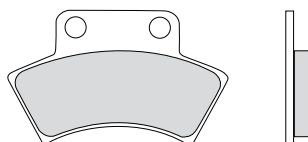
FDB2054 73.5x43.5x7.25mm
