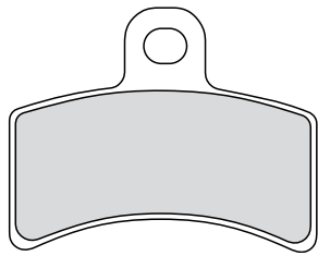
FDB2103 56.9x44.3x6.5mm
