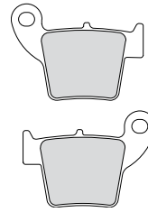
FDB2139 60.2x44.2x9.5mm
