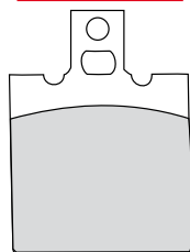
FRP416 40x55x9.3mm
