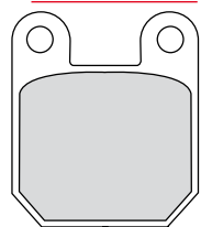
FRP405 36.1x45.1x6mm
