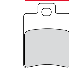
FDB2056 49.1x35.8x7mm
