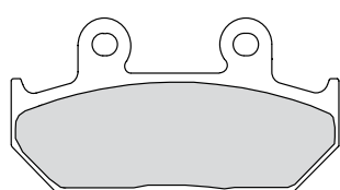
FDB2173 88x46x8.5mm
