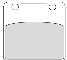
FDB389 58x54x8.7mm
