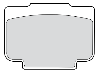
FDB2122 49.8x35.95x8.1mm
