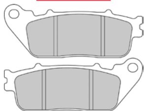
FDB2253 99.3x38.6x8.9mm
