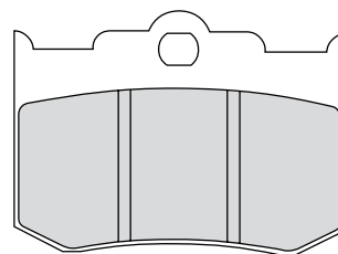
FDB2041 69.4x51.1x11mm
