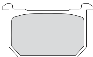
FDB299 68x41x8mm
