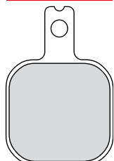
FRP415 33.6x49.7x7mm
