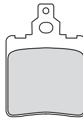
FDB624 35x52x7mm
