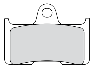
FDB2193 65.8x44.7x11.4mm
