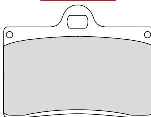
FRP408 70x51x8.3mm
