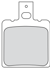
FDB2081 39.8x56.5x8mm
