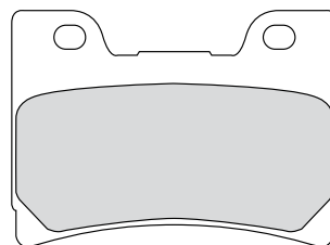
FDB666 75x55x10.9mm
