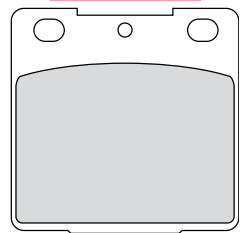
FDB183 54x53x9.5mm
