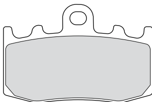
FDB2125 77.6x51.8x8.5mm
