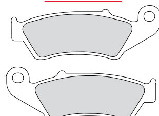
FDB892 94x35x7.7mm
