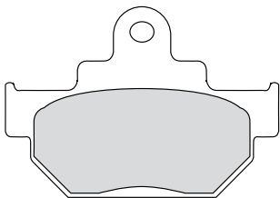
FDB673 77x54x9.4mm
