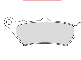
FDB2006 108x41x7.5mm
