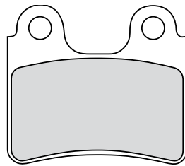
FDB2109 50.1x43.5x6mm
