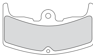
FDB310 92x53x8mm
