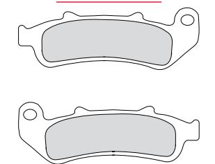
FDB2002 125x44.3x8.8mm
