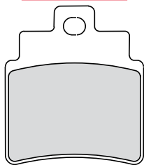
FDB2141 44.6x51.2x7mm
