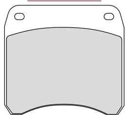
FRP213 59.5x54.4x10.2mm
