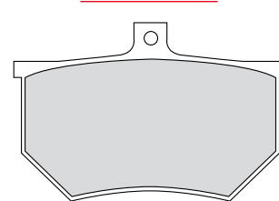
FRP410 84x54x8mm
