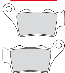
FDB2019 77x40x9.9mm
