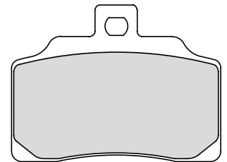
FDB2185 64.1x48.3x8.1mm
