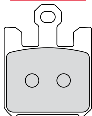
FDB2164 39x49.9x7.9mm
