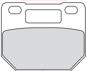
FDB437 53x44x7.5mm
