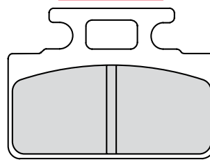
FDB2192 52x36.8x8.2mm
