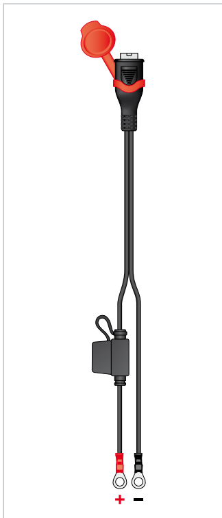
63 0064 Weatherproof Permanent Lead
