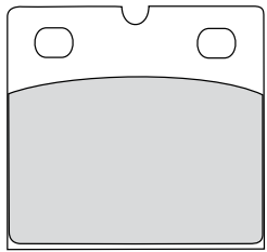
FDB148 56x55x7.6mm
