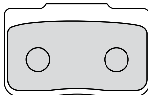
FDB2170 49.8x31.8x8.1mm
