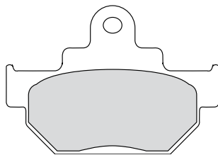
FDB404 77x54x7.1mm
