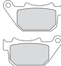
FDB2180 86.4x44.9x10mm
