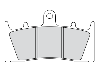
FDB2144 90x52x9.9mm
