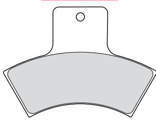
FDB2121 74.2x53.2x7mm
