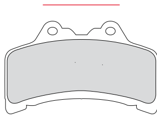
FDB865 132x81.6x9.6mm
