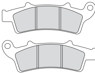
FDB2105 117.5x41.3x8.6mm
