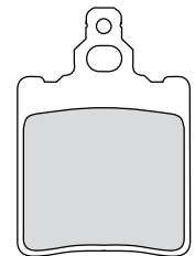
FDB694 35x52x6mm
