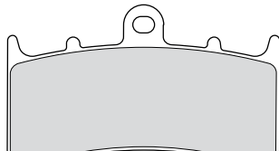
FDB2124 81.65x46.25x9mm
