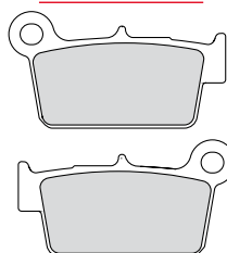
FDB2162 66.9x36x9.4mm
