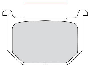
FDB218 78x50x10.5mm
