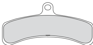
FDB2034 117.1x55.4x8mm
