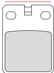
FDB695 37.8x51.1x7mm
