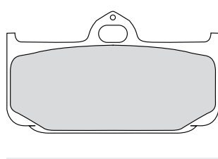
FDB2008 77.6x45.4x8.7mm
