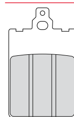
FDB698 44.1x71.6x7.6mm
