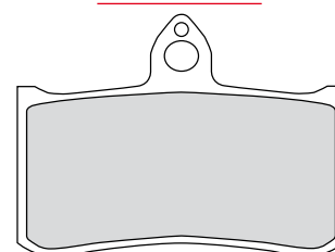
FDB858 69.8x52.5x8.7mm
