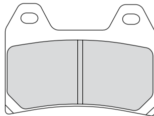
FDB2099 75x55.2x7.6mm
