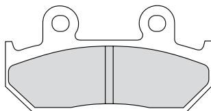
FDB2113 81.2x42x9.5mm
