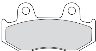
FDB2119 81.3x42.1x9.4mm
