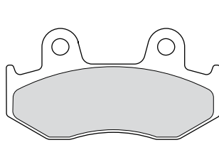
FDB2132 81.2x42.2x8.3mm
