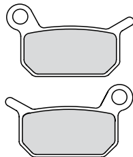
FDB2183 43.6x25.3x5mm
