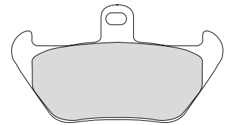
FDB657 100x56x8.3mm
