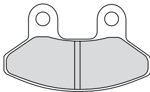
FDB2108 70.2x41.8x8.1mm
