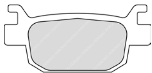
FDB2212 81.8x37.7x9.6mm
