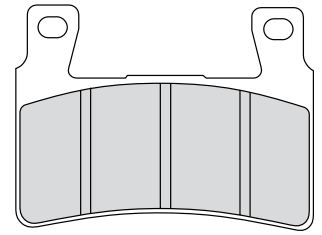
FDB2079 74x55.1x9.0mm
