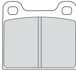
FDB2136 61.8x56.6x11.5mm
