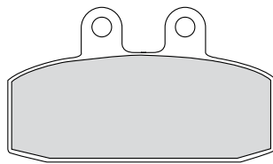
FDB438 79x47x7.4mm
