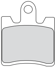
FDB2085 44.8x53.5x8.6mm
