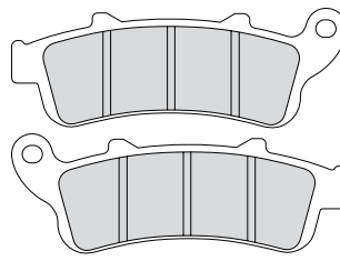
FDB2075 115.1x41x9.4mm
