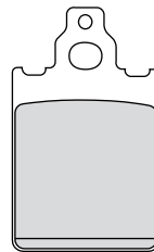
FDB2100 31.7x51.1x6mm
