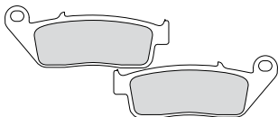
FDB664 101x35x9.8mm
