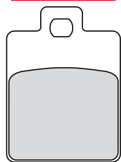
FDB2057 49.1x35.8x7mm
