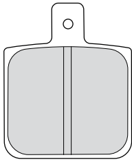
FDB2135 50.4x60.9x12mm
