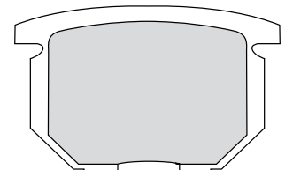
FDB217 72x45x11.4mm
