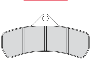
FDB887 117.1x58.8x8mm
