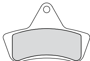
FDB2175 67.8x45.1x7.6mm
