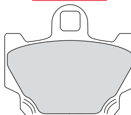
FDB311 68.1x58.7x8.4mm
