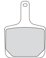
FDB2189 57.9x78.3x11.6mm
